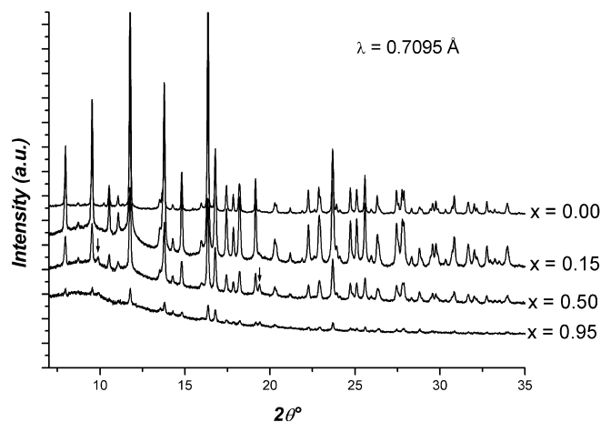
Fig. 9 Synchrotron powder diffraction pattern of LT-LiCoPO 4 cathode during charging the cell
