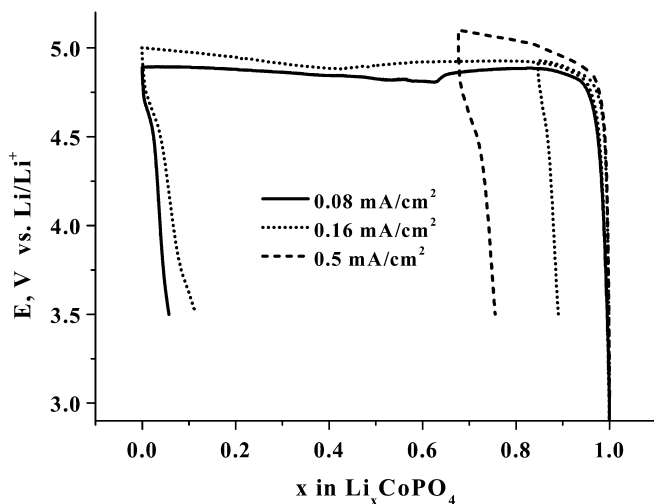
Fig. 2 First charge–discharge curves for HT-LiCoPO 4 in a Swagelok cell with various current densities
