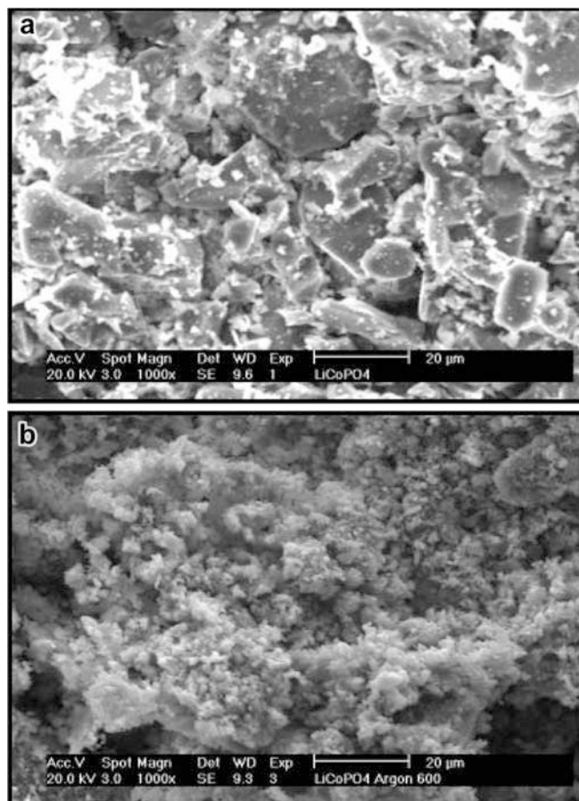
Fig. 1a,b SEM images of \text{LiCoPO}_4 samples prepared by a HT synthesis and b LT synthesis
