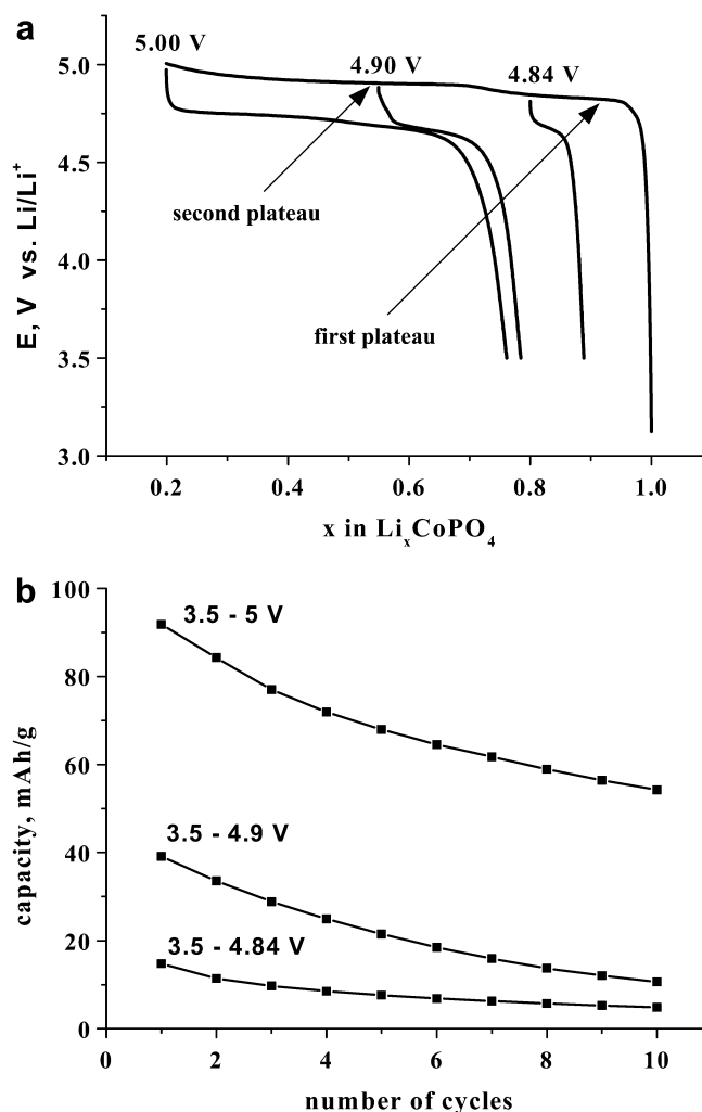
Fig. 7a,b First charge–discharge curves for LT- \text{LiCoPO}_4 , charged to the different cut-off voltages (a) and discharge capacity versus cycle number on cycling in the selected voltage ranges (b)
